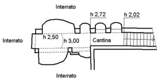
PIANO SEMINTERRATO
